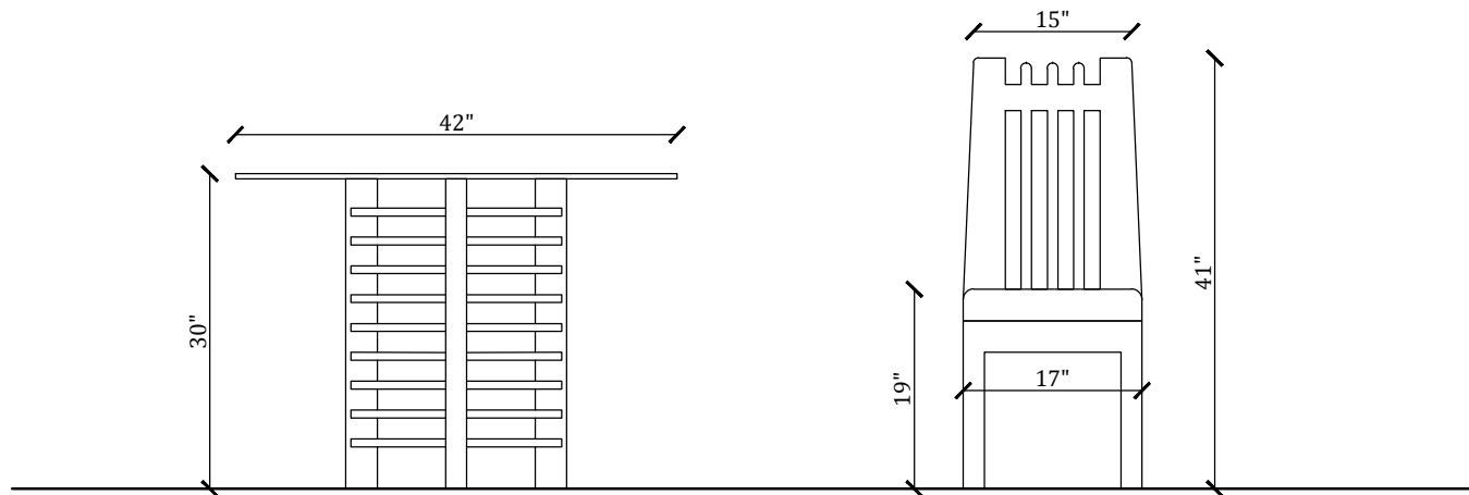
DINING TABLE FRONT VIEW
